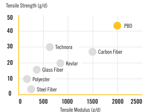
MODULUS & TENSILE STRENGTH (Based on BRP Dynamometer Testing)
